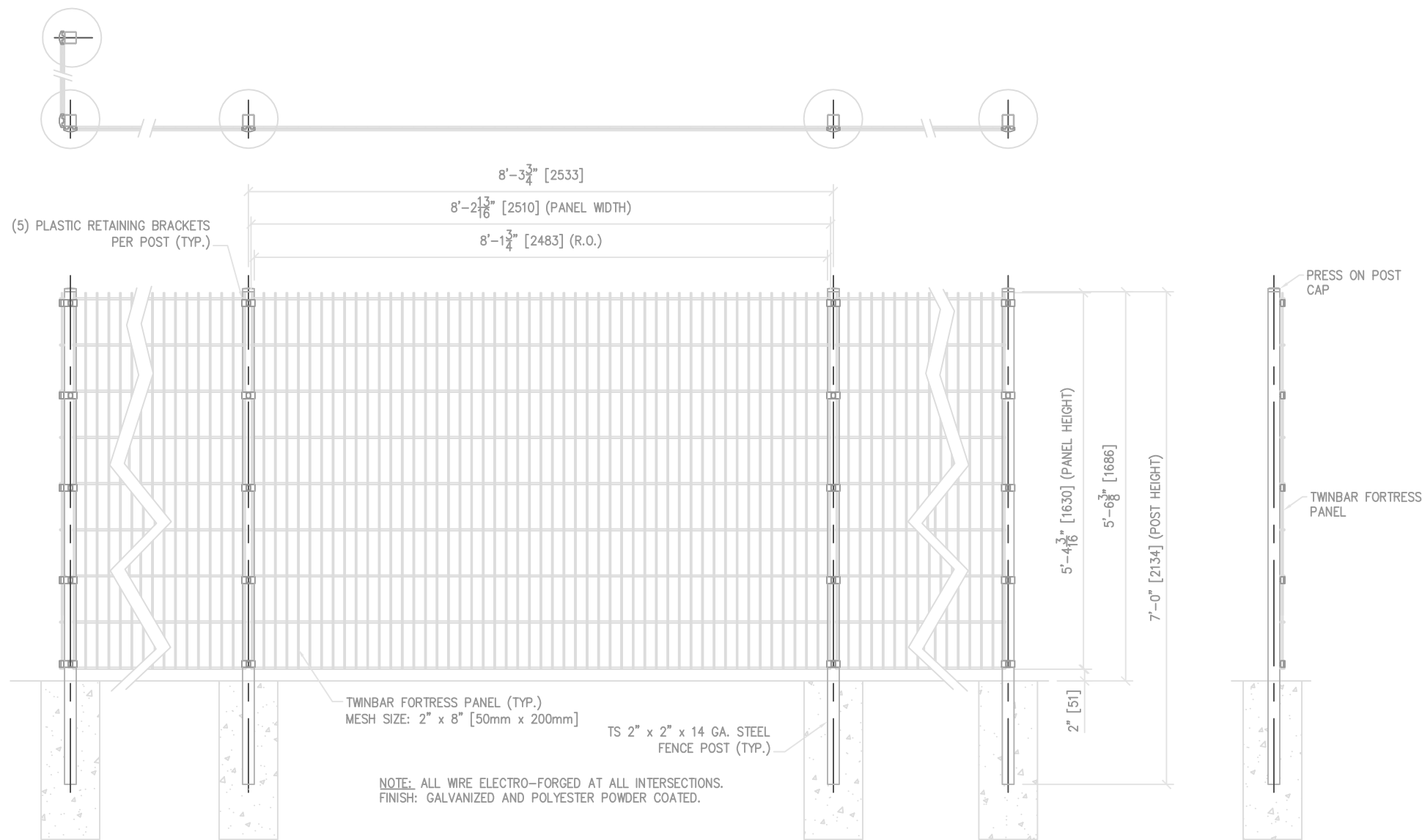
1 TYPICAL 5'-0" HIGH TWINBAR FORTRESS PANEL DETAILS SK1 SCALE: 1/2"=1'-0"
