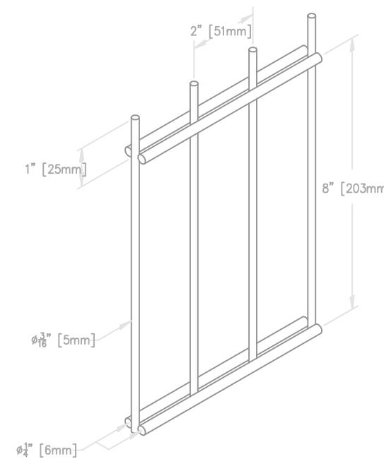
3 TWINBAR FORTRESS PANEL ISOMETRIC SK1 SCALE: 3"=1'-0"
