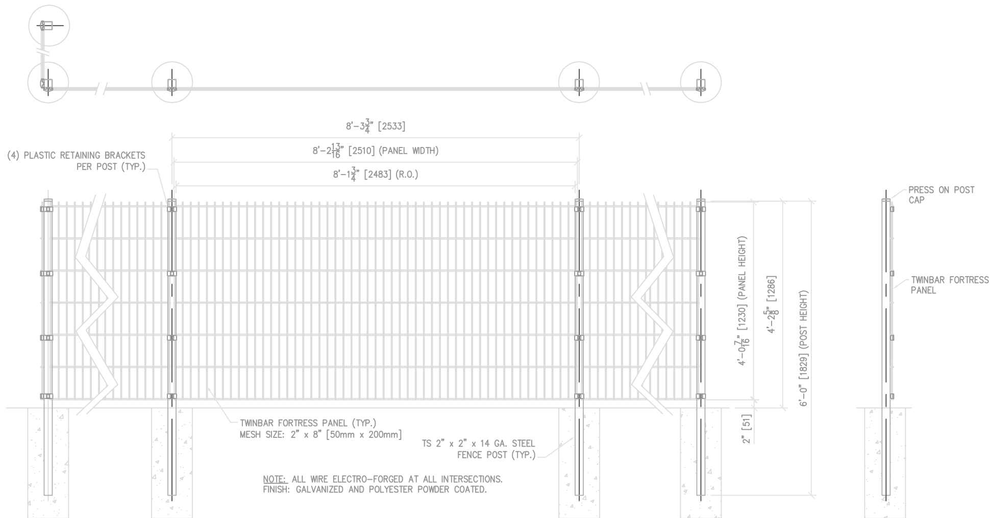
1 TYPICAL 4'-0" HIGH TWINBAR FORTRESS PANEL DETAILS SK1 SCALE: 1/2"=1'-0"
