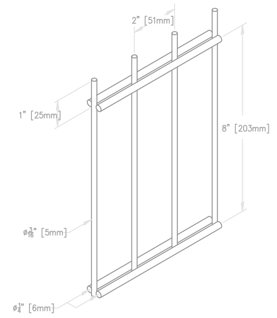
3 TWINBAR FORTRESS PANEL ISOMETRIC SK1 SCALE: 3"=1'-0"
