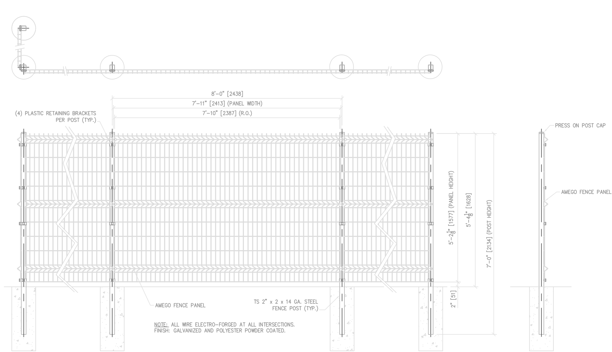
1 TYPICAL 5'-0" HIGH AMEGO PANEL DETAILS SK1 SCALE: 1/2"=1'-0"
