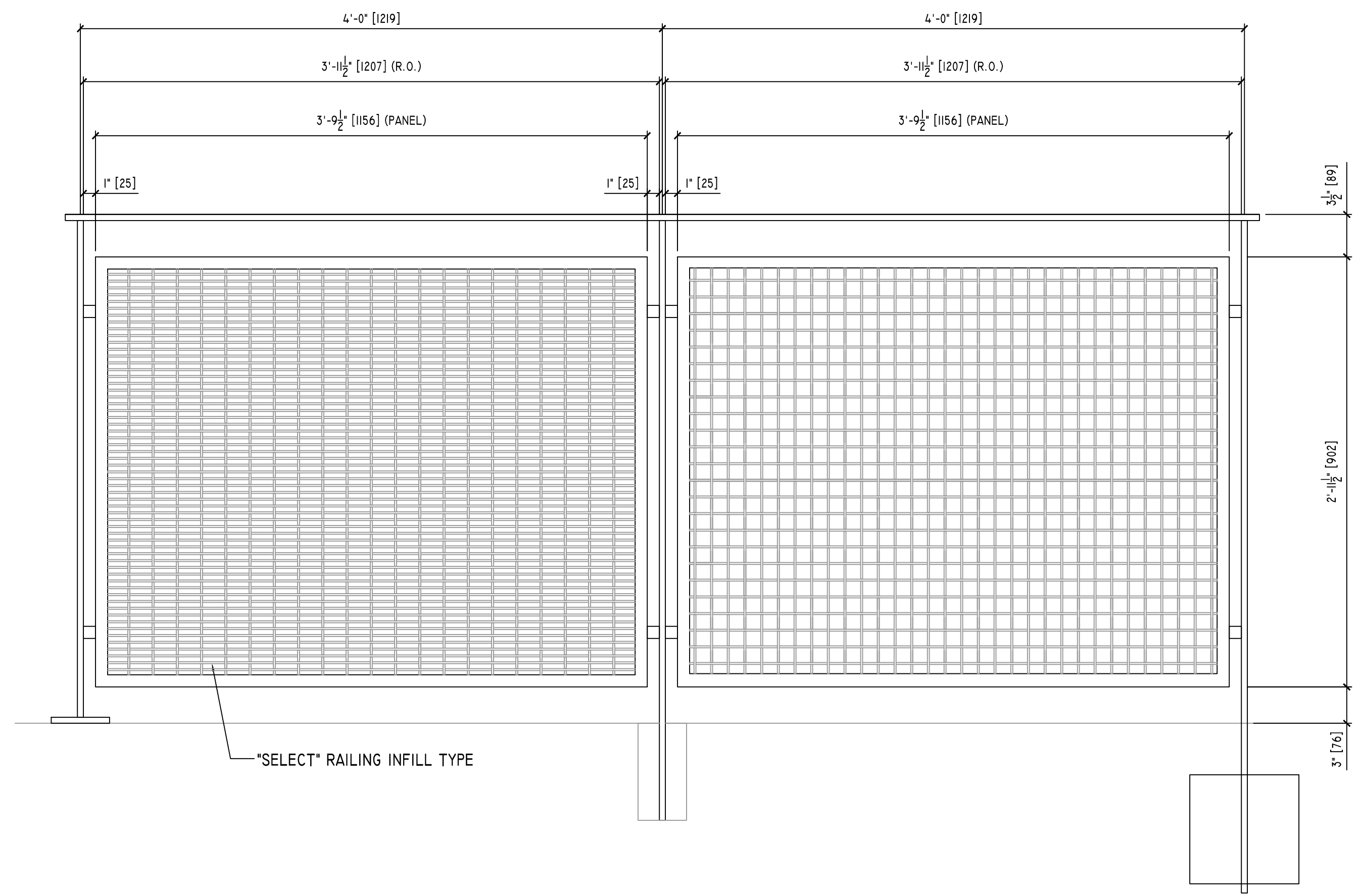
1 TYPICAL "SELECT" WOVEN MESH RAILING SYSTEM AI SCALE: 1"=1'-0"
