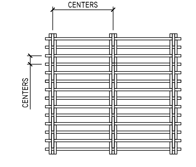
3 SELECT STYLE 1500 AI RETANGULAR DOUBLE WEAVE MESH SCALE: 3"=1'-0"
