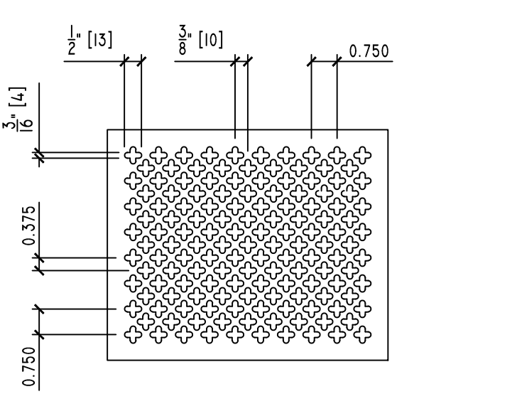
10 FULL CLOVERLEAF DECORATIVE AI SCALE: 3"=1'-0"
