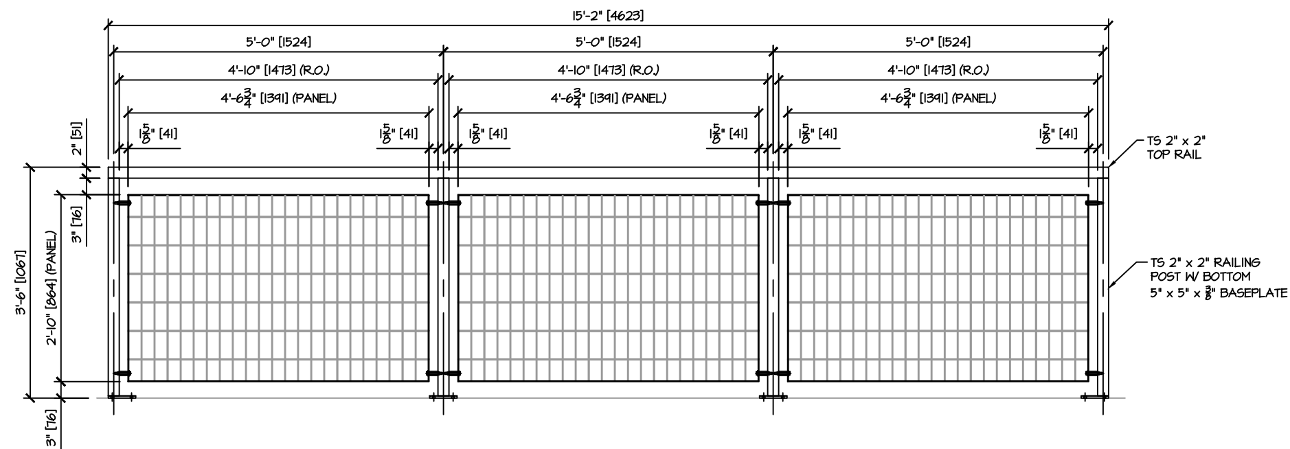
1 TYPICAL GRIGLIATO RAILING SYSTEM W/ SPACERS & TOP RAIL SKI SCALE: 1/2"=1'-0"
